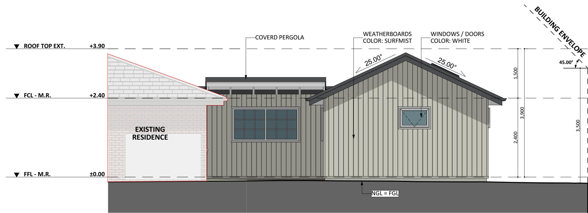
SOUTH-WEST ELEVATION - CD
